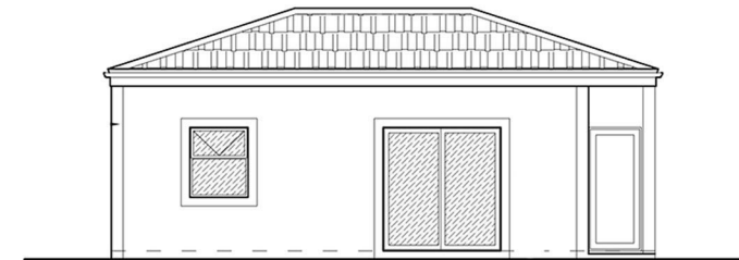
west elevation I scale 1:100
