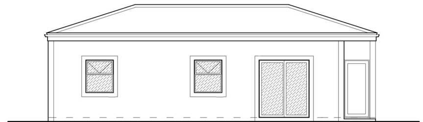
east elevation I scale 1:100
